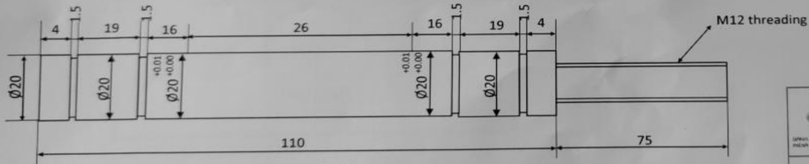
Shaft
