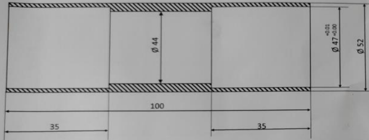
Roll shell
