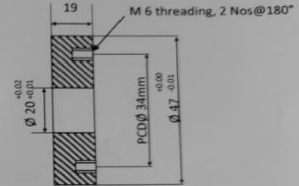
Sealing Bush
